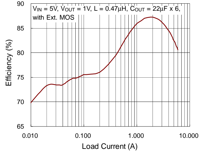
BUCK3 Efficiency vs. Load Current
