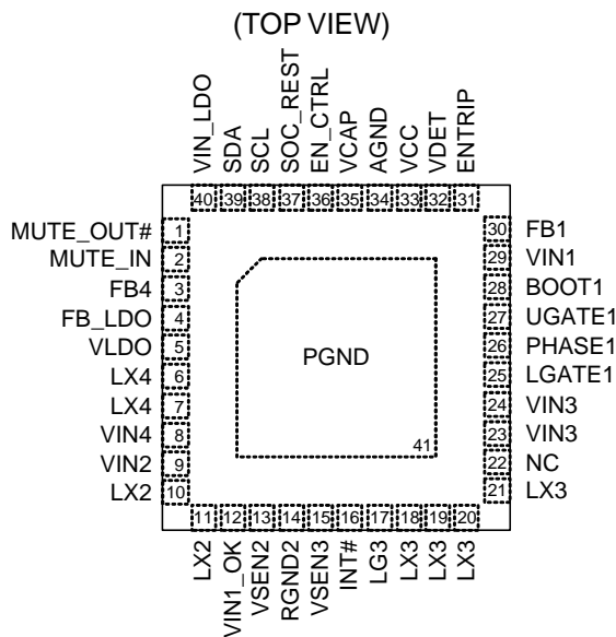
WQFN-40L 5x5
