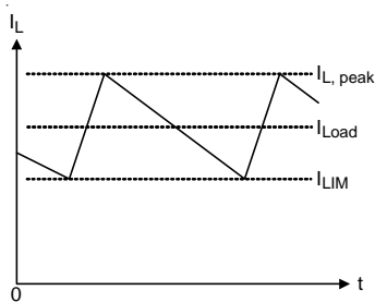
Figure 4. “Valley” Current Limit
