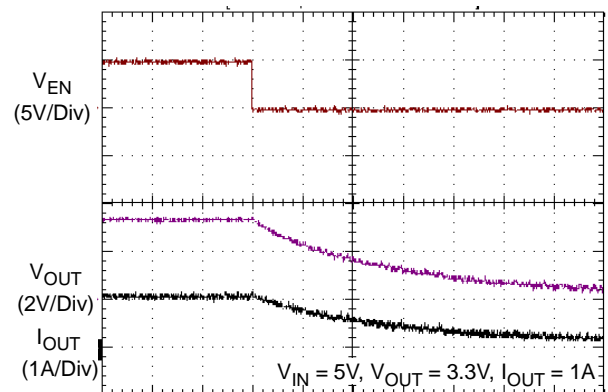
Time (10µs/Div)
