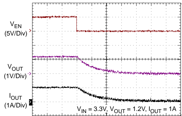
Time (10µs/Div)
