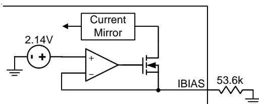
Figure 4. IBIAS Setting
