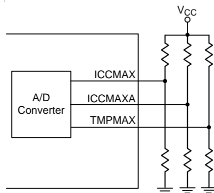
Figure 5. ADC Pins Setting
